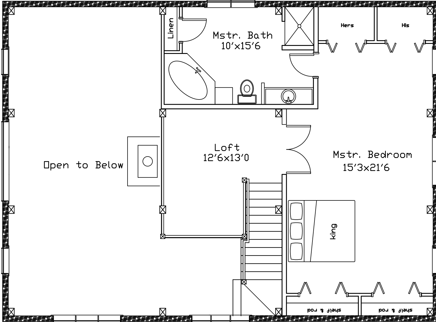
Second Floor Plan 773 sf
